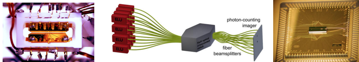
Figure 7. (left) A small programmable (5-qubit) trapped ion quantum computer. (Monroe group, University of Maryland and Joint Quantum Institute). (center). Photonic interconnects to connect quantum memory modules (Credit: Kenneth R Brown, Jungsang Kim & Christopher Monroe). (right) Advanced microfabricated ion traps from Sandia National Laboratories (Image courtesy of Duke University).
