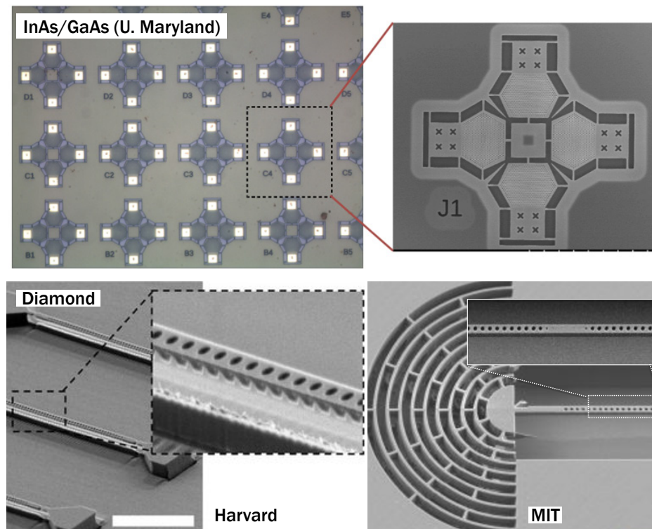
Figure 10. Quantum emitters and spin memories are being scaled up to on-chip networks. (Top) Cavity-waveguide networks for InAs/GaAs quantum dots. (Credit: Waks group, University of Maryland). Bottom: Diamond cavity-waveguide systems with triangular (bottom left) and rectangular (bottom right) nanobeams for NV and SiV memories. (MIT and Harvard)
